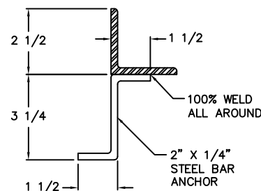
ANCHOR DETAIL
