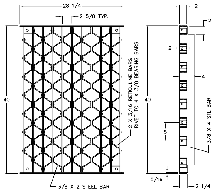
GRATE TOP VIEW
