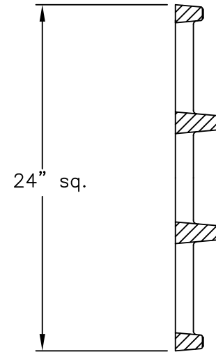
GRATE SECTION
