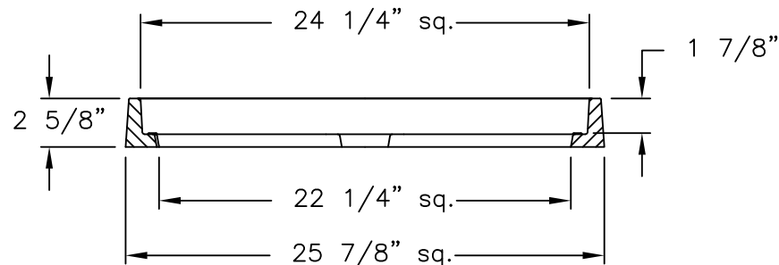
FRAME SECTION
