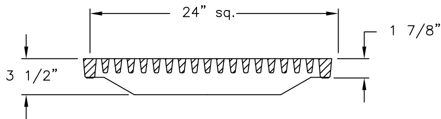
GRATE SECTION
