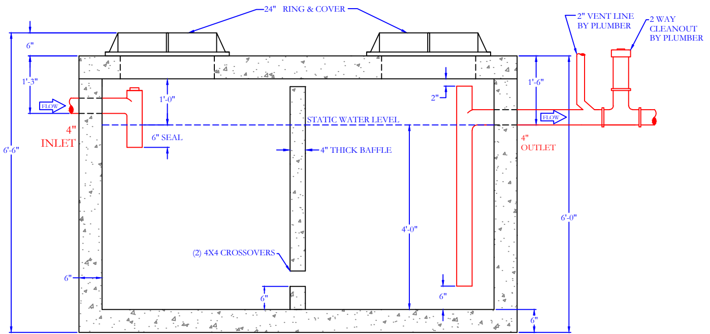
ELEVATION VIEW
