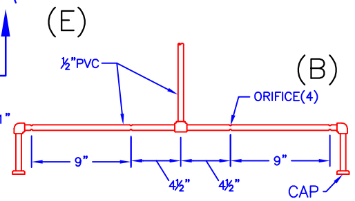
AIR DIFFUSER
