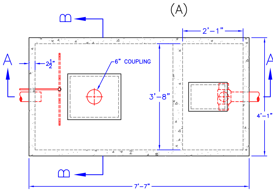
TOP PLAN
